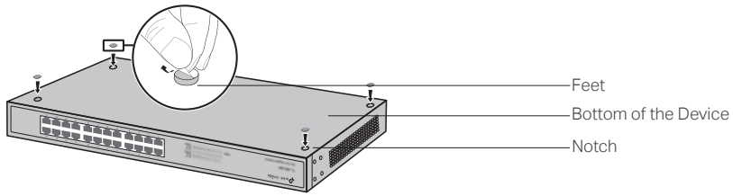
Figure 2-1 Desktop Installation
