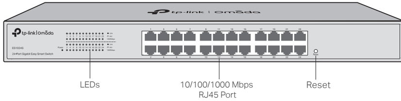
Figure 1-4 Front Panel of ES1024G
