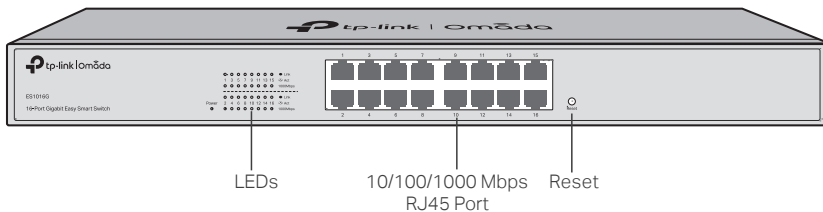
Figure 1-2 Front Panel of ES1016G
