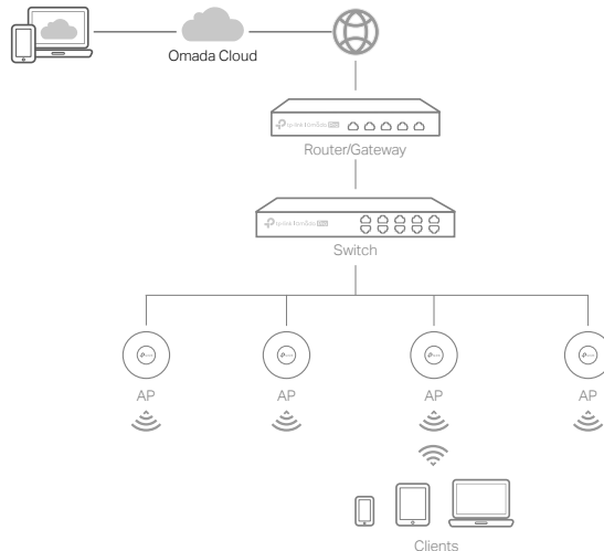
Figure 4-3 Manage the network via Omada Pro Cloud-Based Controller
