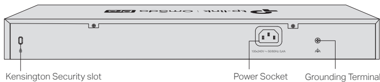
Figure 1-3 Rear Panel
