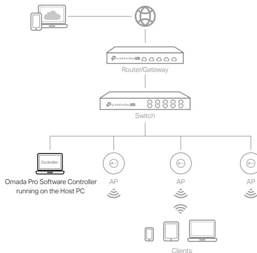
Figure 4-2 Manage the network via Omada Pro Software Controller
