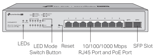
Figure 1-1 Front Panel of S4500-8GHP2F
